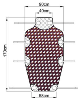
5467.94 Mesh Sling
